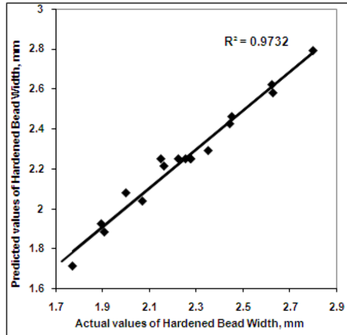
Figure.4. Actual/Predicted values of Hardened Bead Width.
