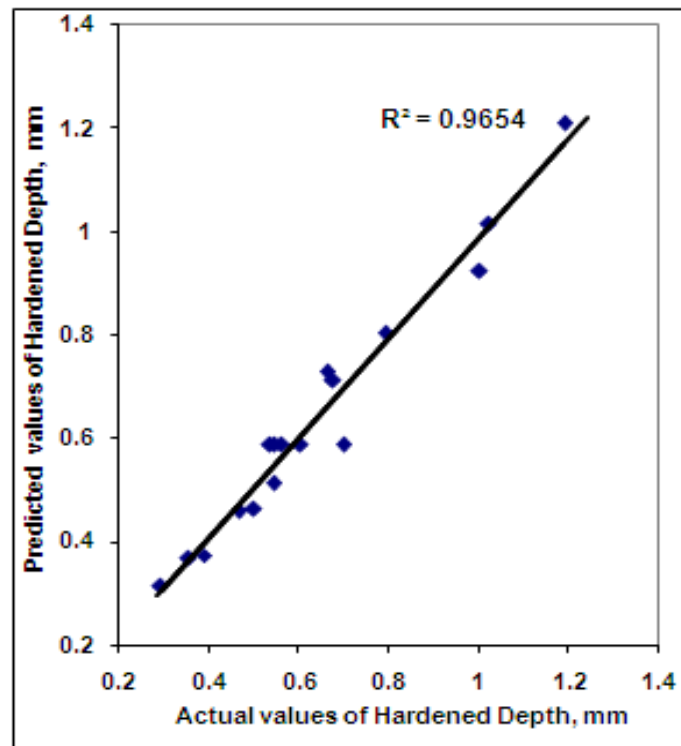
Figure.5. Actual/Predicted values of Hardened Depth.
