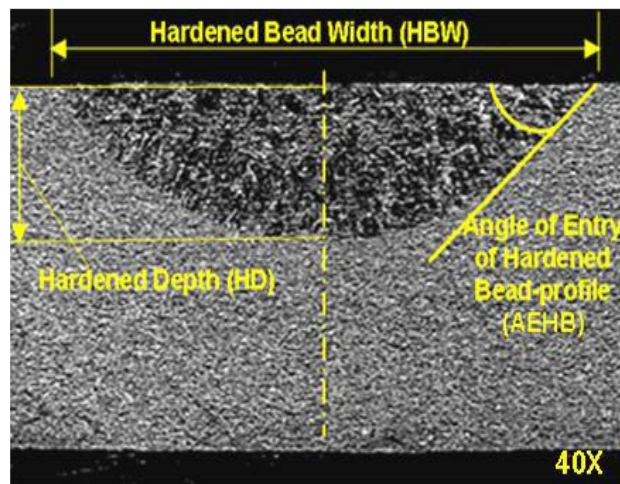
Figure 3. Microstructure of Hardened- Bead Profile with parameters, HBW, HD and AEHB (WRI 2008).
