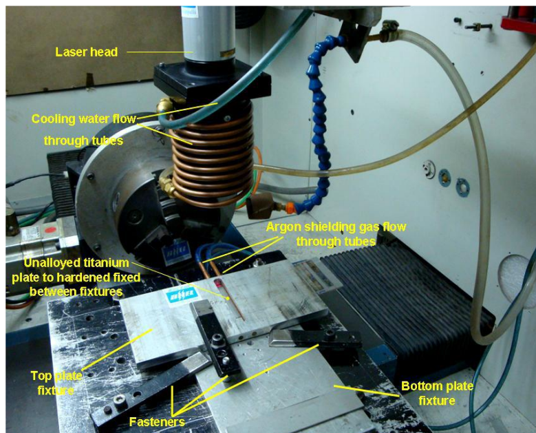
Figure.1. Solid state Nd:YAG Laser source at WRI used for experimental work (WRI 2008).
