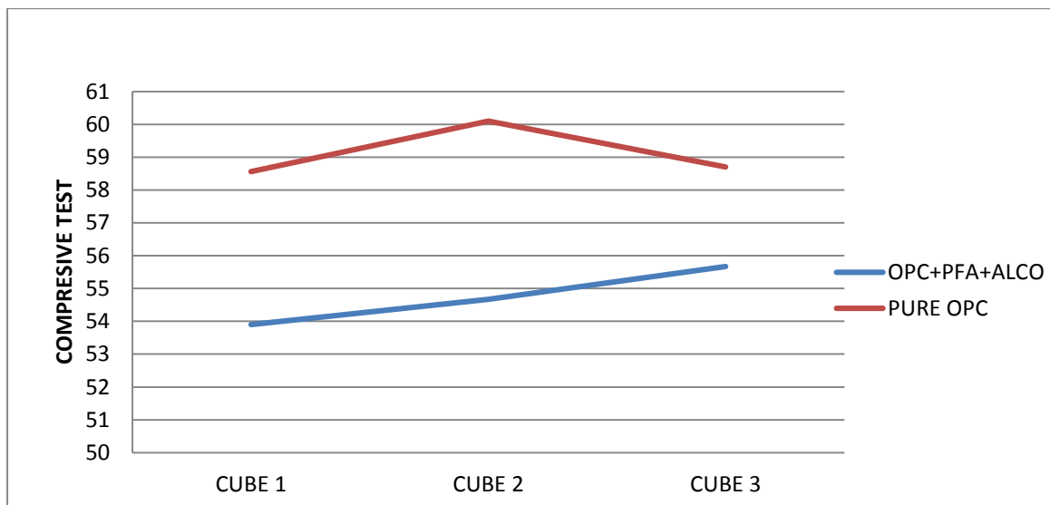
Figure 2: Variation in compressive strength at 7 days.
