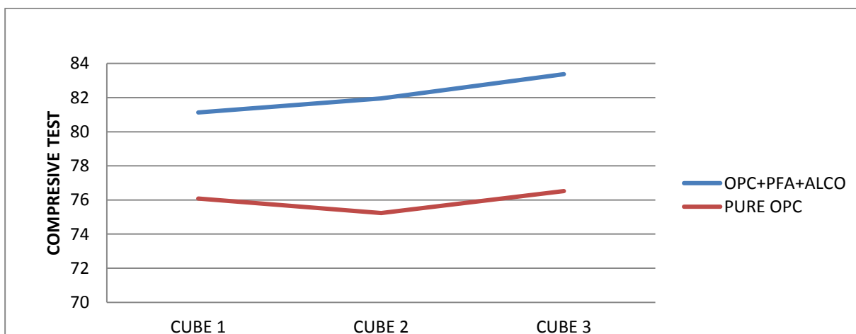
Figure 3: Variation in compressive strength at 28 days.
