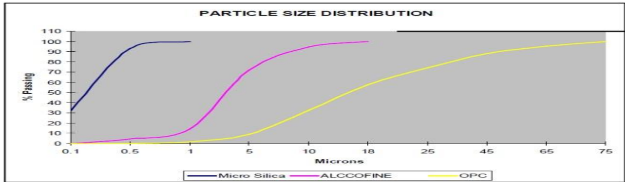
Figure. 1 Particle Size Distribution
