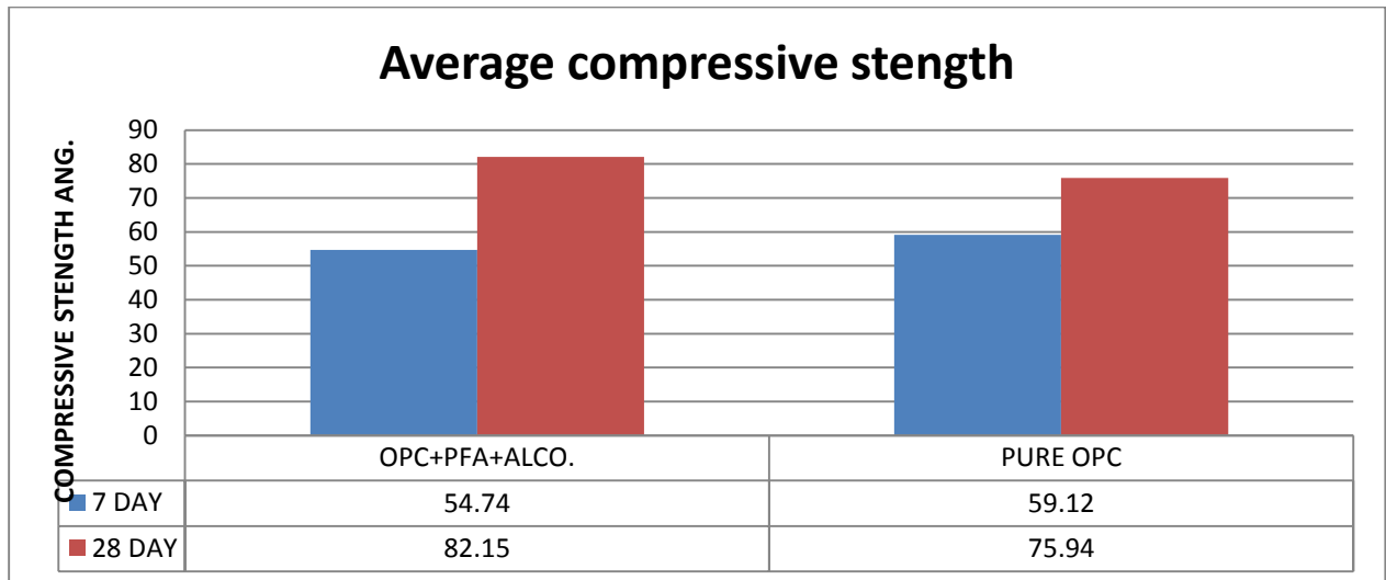
Figure 4: Average compressive strength at 7 and 28 days.
