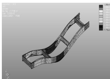
Displacement in Y direction
