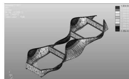
Displacement in Z direction
